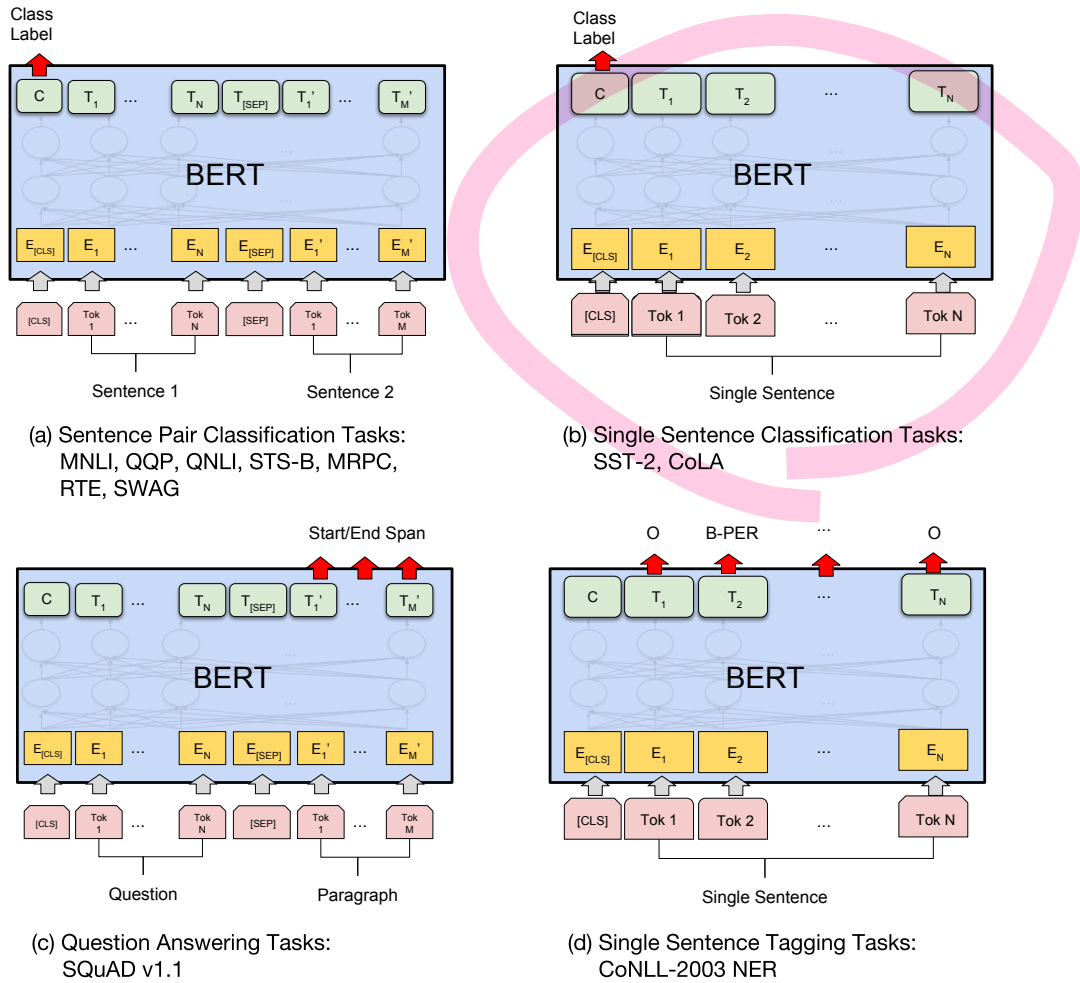
Figure 4: Illustrations of Fine-tuning BERT on Different Tasks.
